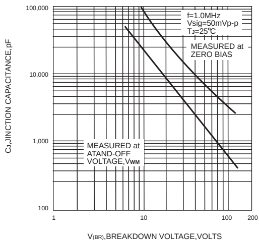
FIG. 4-TYPICAL JUNCTION CAPACITANCE
