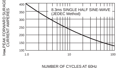
FIG.6-MAXIMUM NON-REPETITIVE FORWARD SURGE CURRENT
