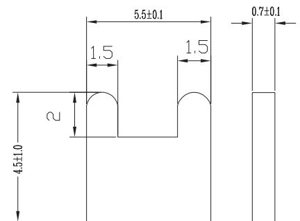
Terminal diagram
