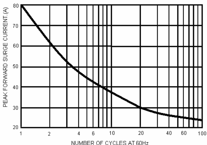
FIG.1-MAXIMUM NONO-REPETITIVE FORWARD SURGE CURRENT PER BRIDGE ELEMNT
